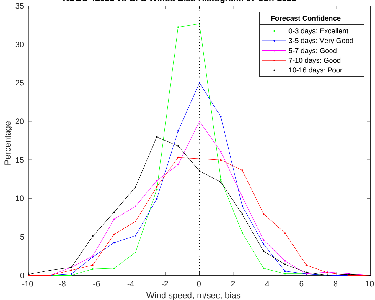
NDBC 42036 vs GFS Winds Bias Histogram: 07-Jun-2025
