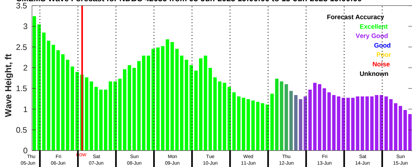
CMEMS Wave Forecast for NDBC 42036 from 05-Jun-2025 19:00:00 to 15-Jun-2025 19:00:00
