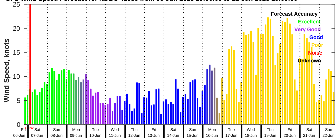
GFS Wind Speed Forecast for NDBC 42036 from 06-Jun-2025 19:00:00 to 22-Jun-2025 19:00:00
