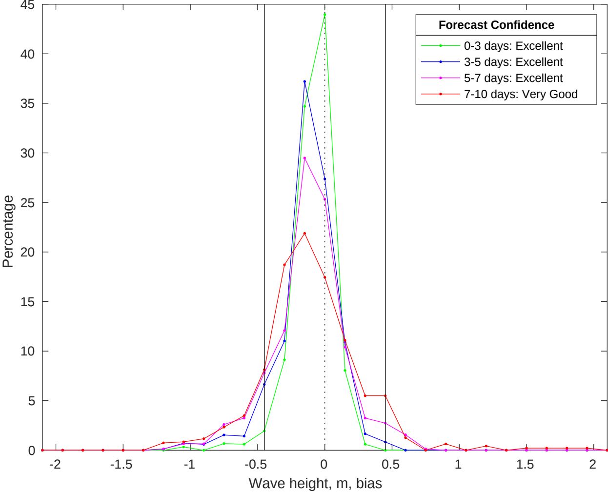
NDBC 42040 vs CMEMS Waves Bias Histogram: 07-Jun-2025
