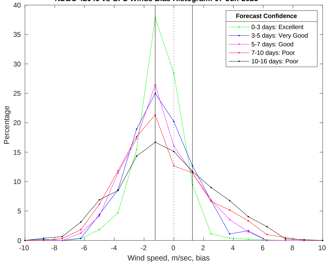
NDBC 42040 vs GFS Winds Bias Histogram: 07-Jun-2025
