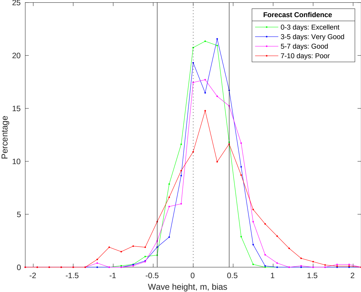
NDBC 46011 vs CMEMS Waves Bias Histogram: 07-Jun-2025
