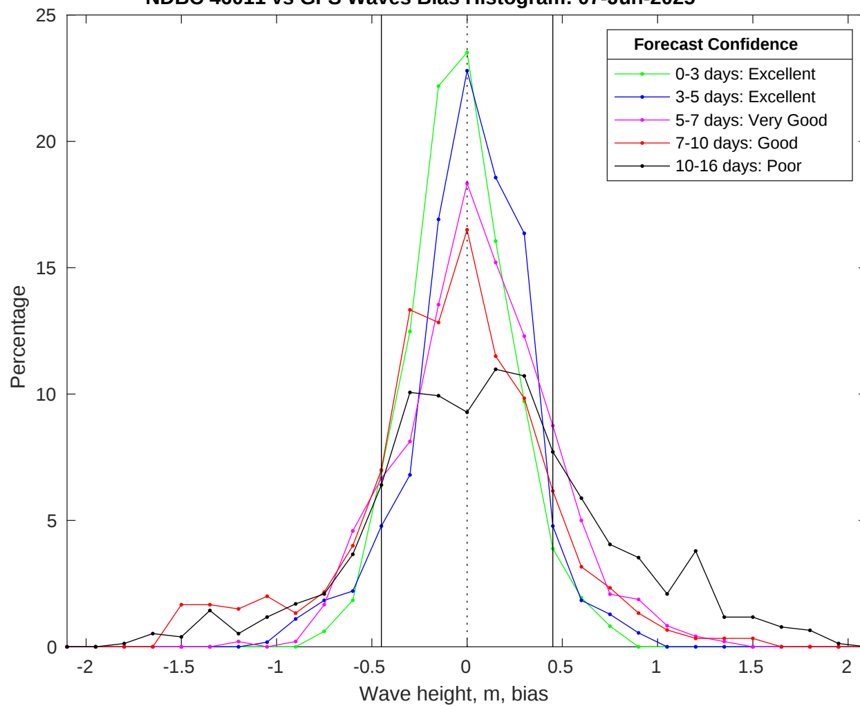
NDBC 46011 vs GFS Waves Bias Histogram: 07-Jun-2025
