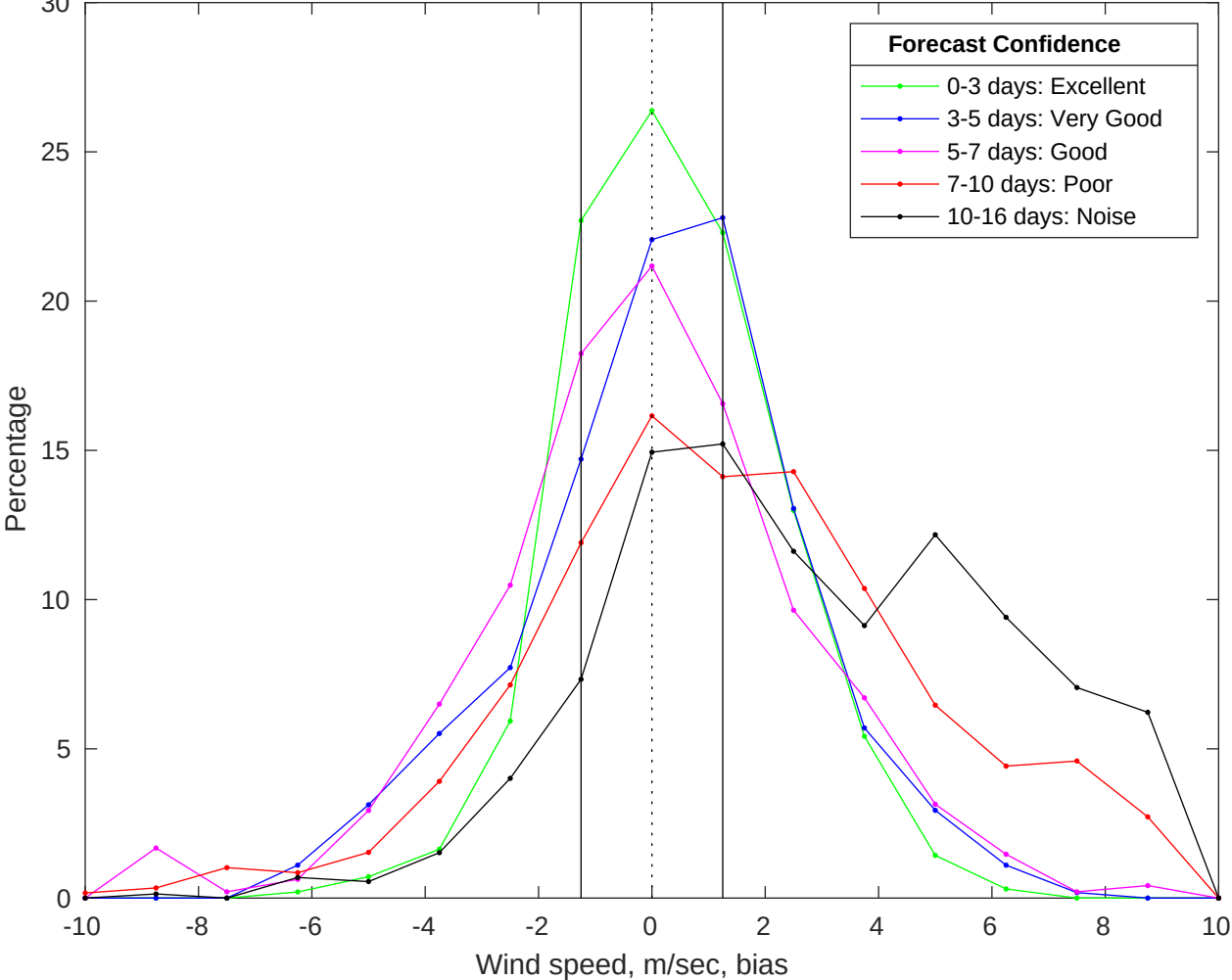
NDBC 46011 vs GFS Winds Bias Histogram: 07-Jun-2025
