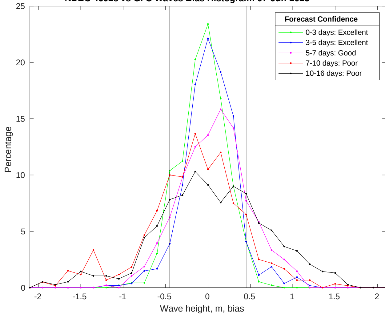
NDBC 46028 vs GFS Waves Bias Histogram: 07-Jun-2025
