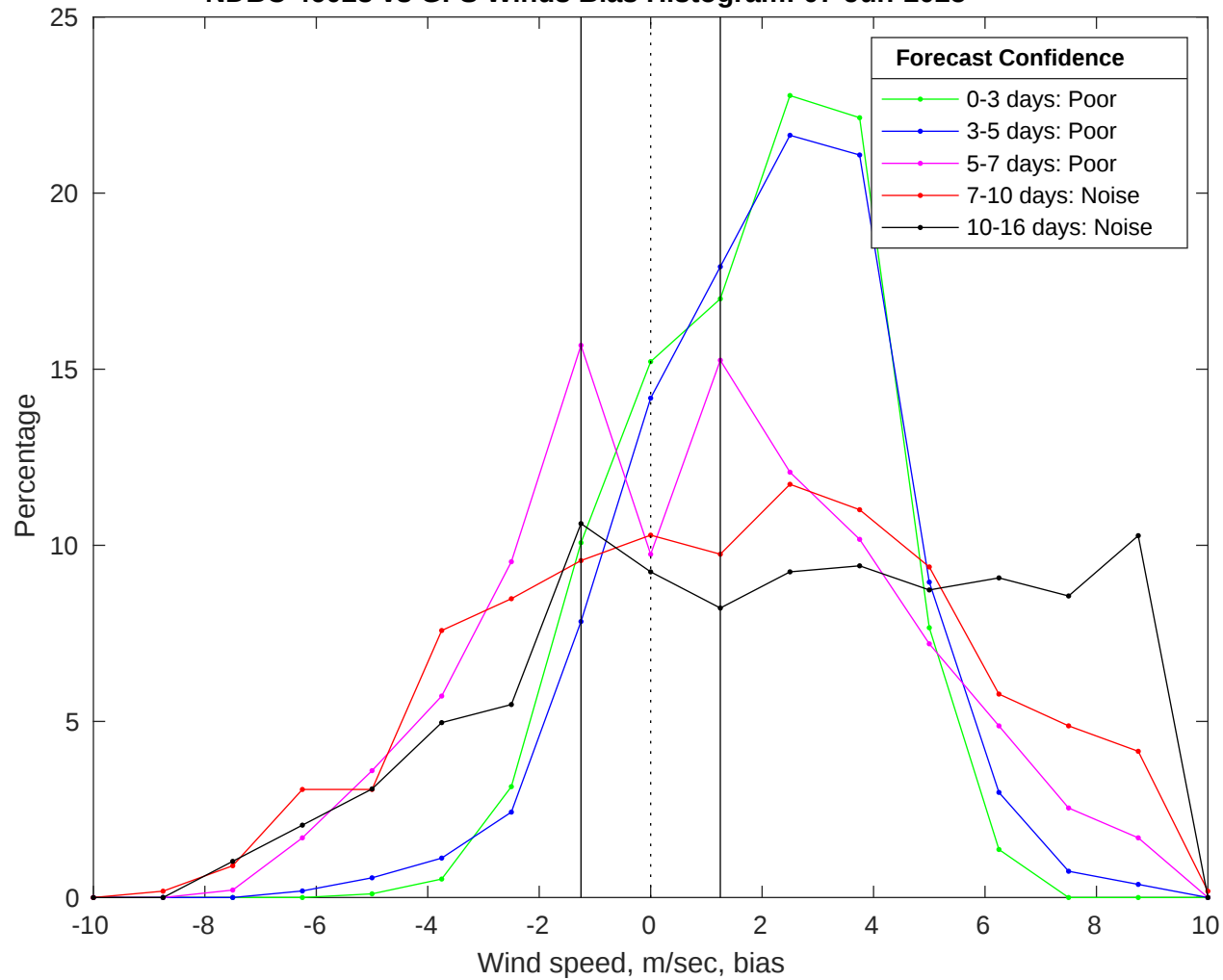
NDBC 46028 vs GFS Winds Bias Histogram: 07-Jun-2025
