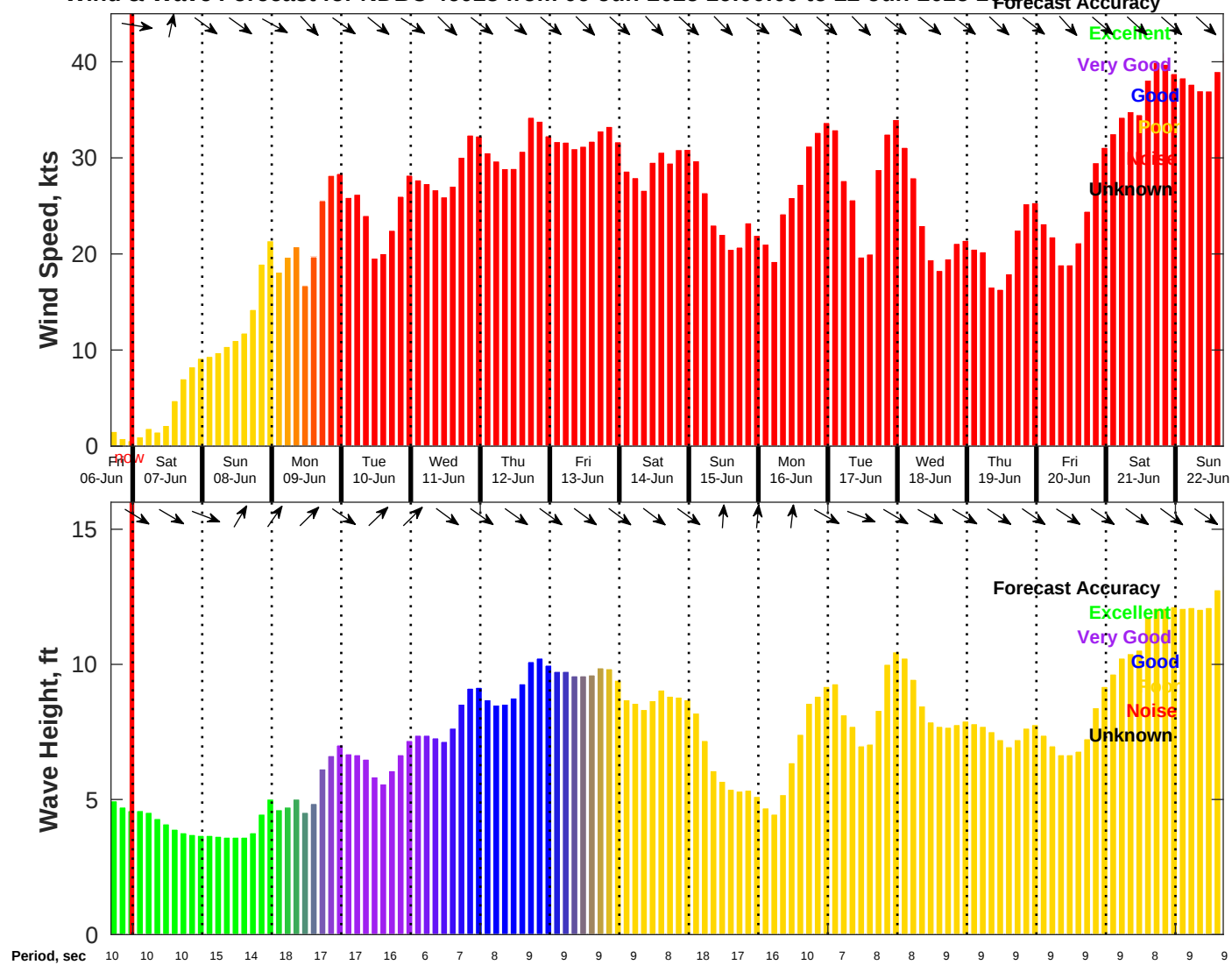
Wind & Wave Forecast for NDBC 46028 from 06-Jun-2025 16:00:00 to 22-Jun-2025 16:00:00
