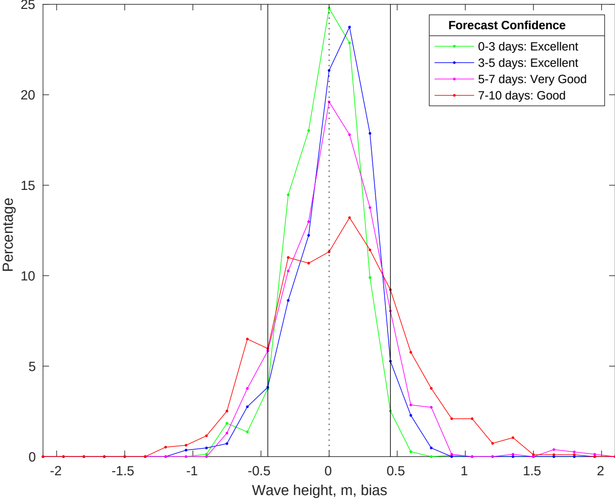
NDBC 46054 vs CMEMS Waves Bias Histogram: 07-Jun-2025
