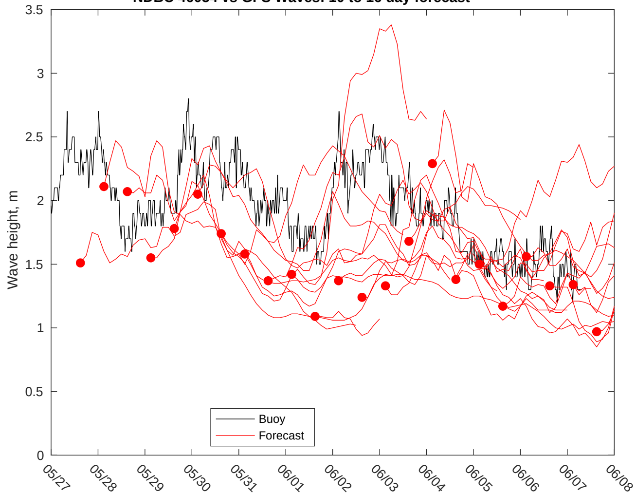
NDBC 46054 vs GFS Waves: 10 to 16 day forecast
