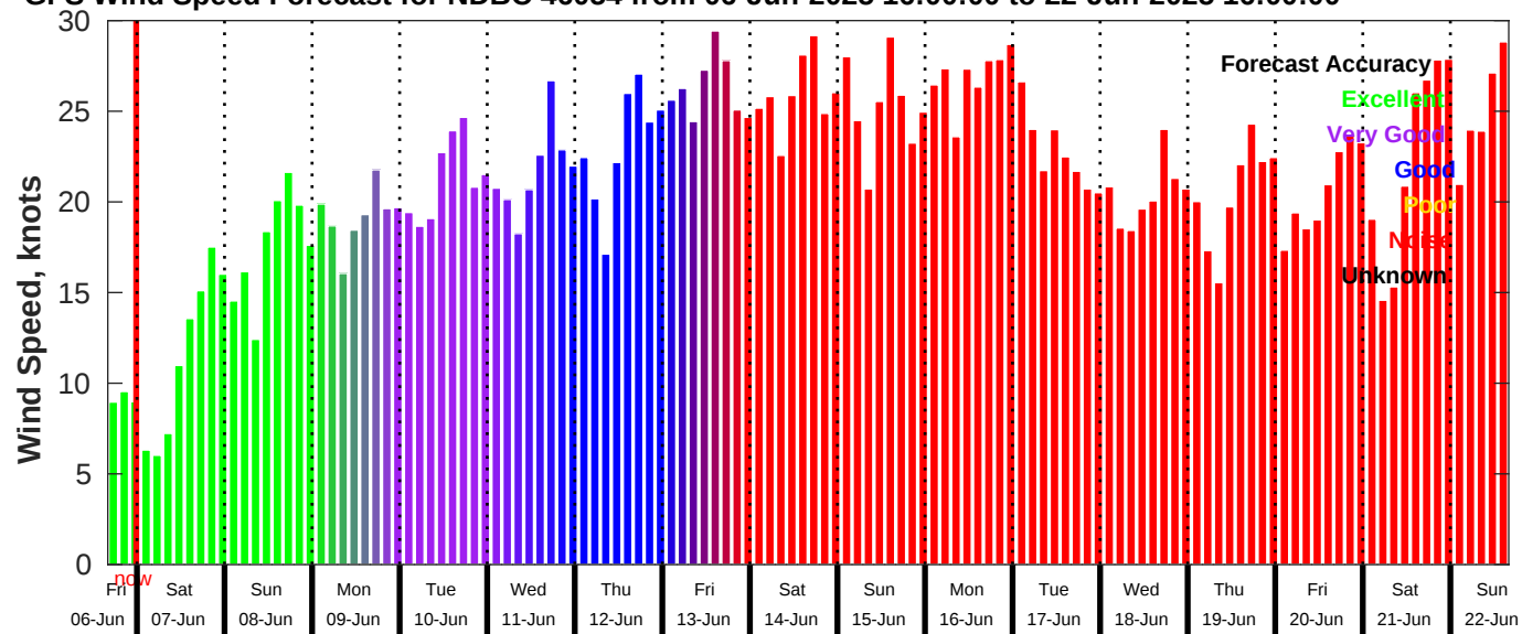
GFS Wind Speed Forecast for NDBC 46054 from 06-Jun-2025 16:00:00 to 22-Jun-2025 16:00:00
