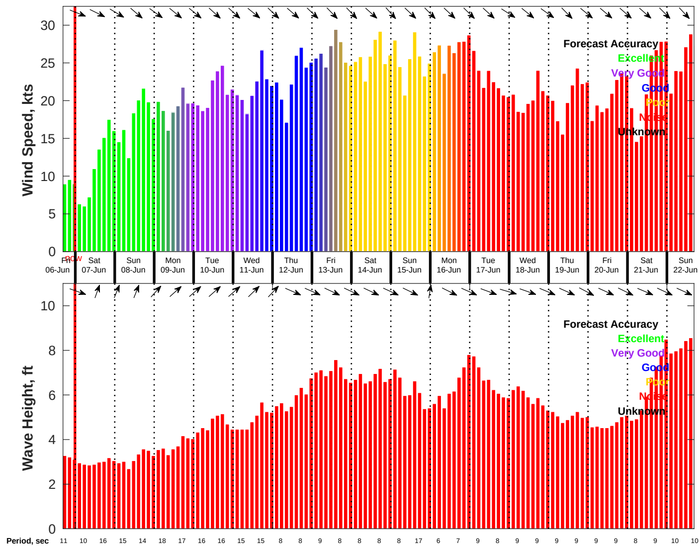
Wind & Wave Forecast for NDBC 46054 from 06-Jun-2025 16:00:00 to 22-Jun-2025 16:00:00
