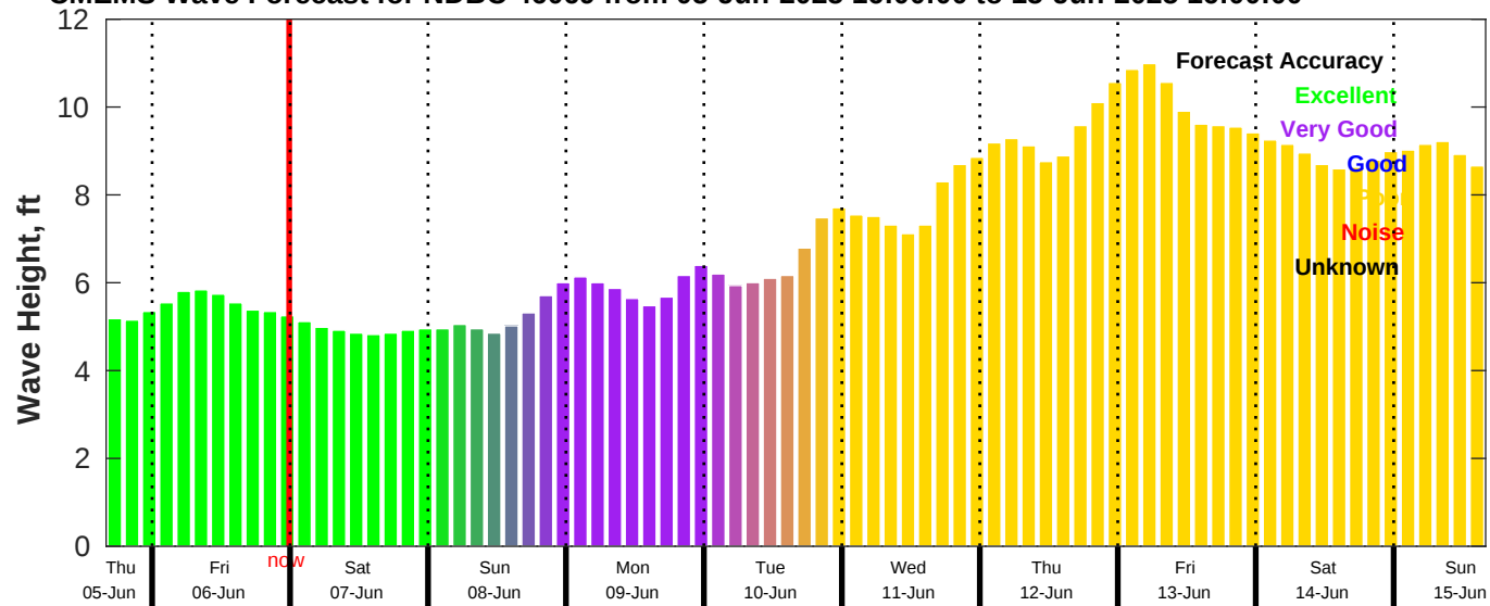
CMEMS Wave Forecast for NDBC 46069 from 05-Jun-2025 16:00:00 to 15-Jun-2025 16:00:00
