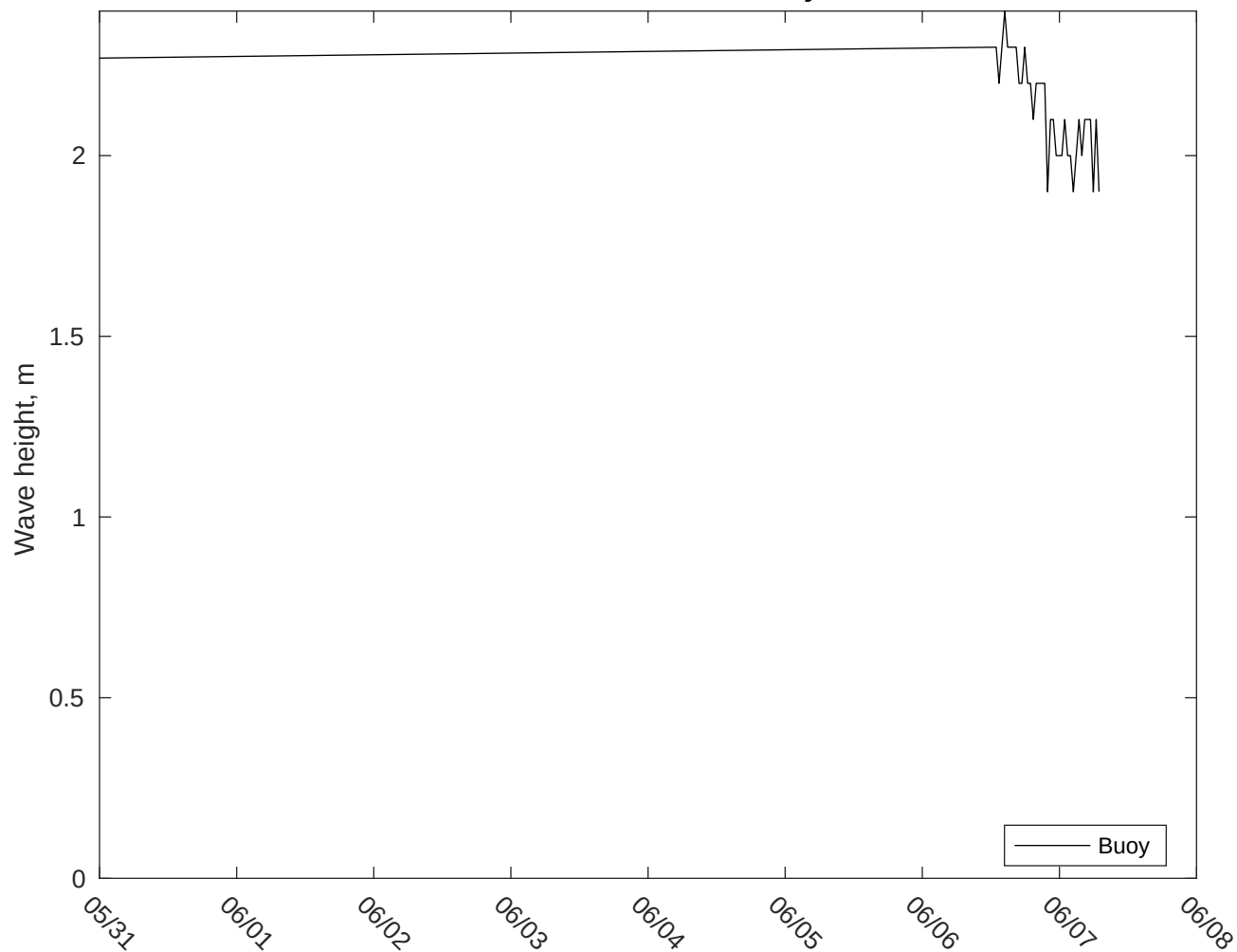
NDBC 51209 vs CMEMS Waves: 10 to 16 day forecast
