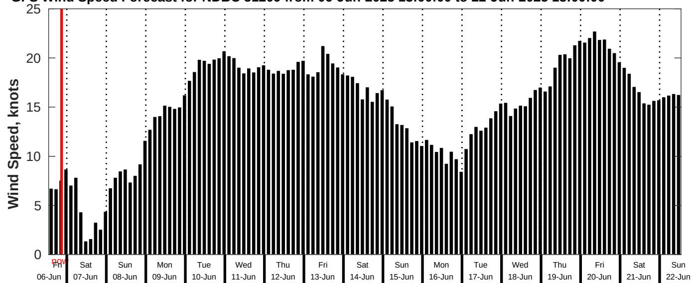
GFS Wind Speed Forecast for NDBC 51209 from 06-Jun-2025 13:00:00 to 22-Jun-2025 13:00:00
