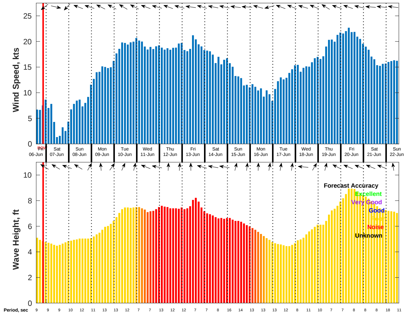
Wind & Wave Forecast for NDBC 51209 from 06-Jun-2025 13:00:00 to 22-Jun-2025 13:00:00
