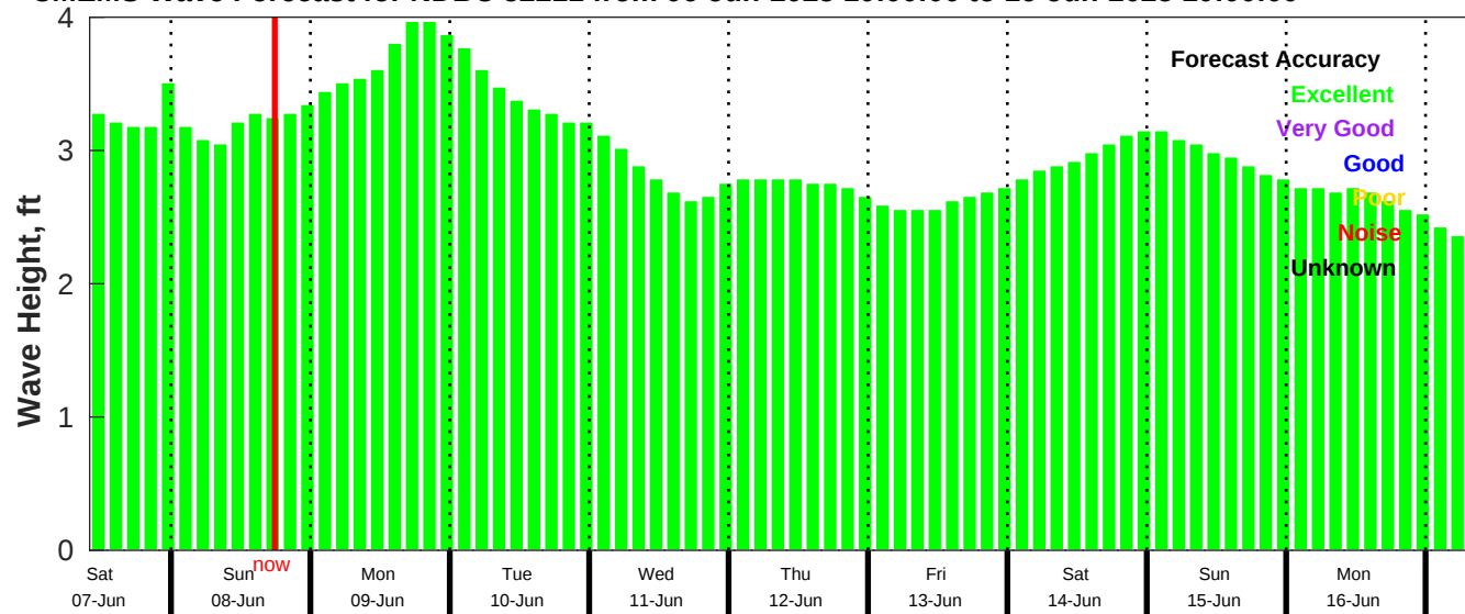
CMEMS Wave Forecast for NDBC 52211 from 06-Jun-2025 10:00:00 to 16-Jun-2025 10:00:00
