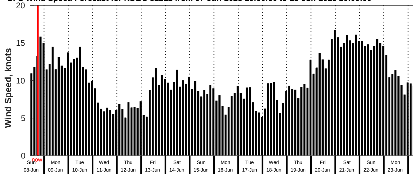
GFS Wind Speed Forecast for NDBC 52211 from 07-Jun-2025 10:00:00 to 23-Jun-2025 10:00:00
