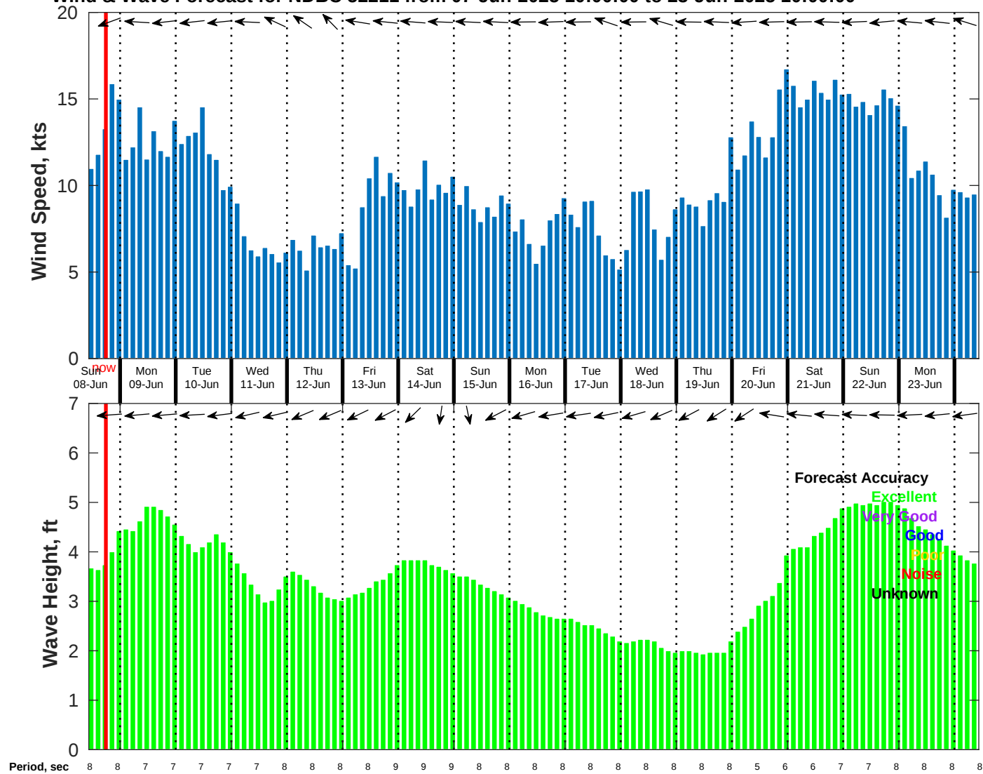
Wind & Wave Forecast for NDBC 52211 from 07-Jun-2025 10:00:00 to 23-Jun-2025 10:00:00
