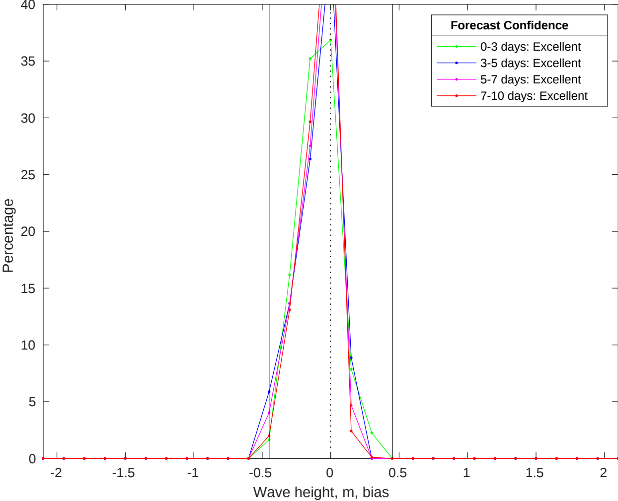
NDBC 52212 vs CMEMS Waves Bias Histogram: 07-Jun-2025
