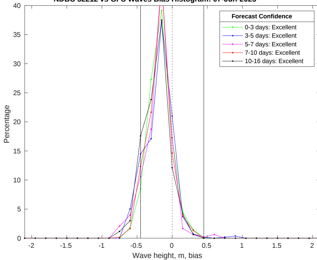
NDBC 52212 vs GFS Waves Bias Histogram: 07-Jun-2025
