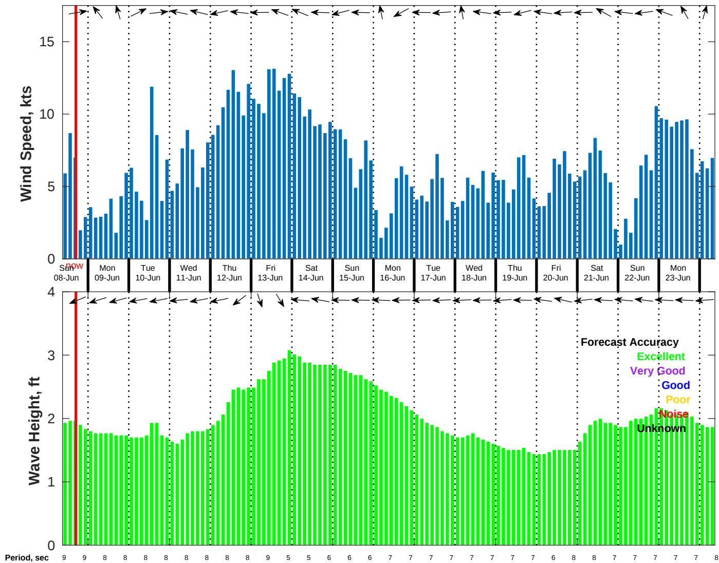
Wind & Wave Forecast for NDBC 52212 from 07-Jun-2025 09:00:00 to 23-Jun-2025 09:00:00
