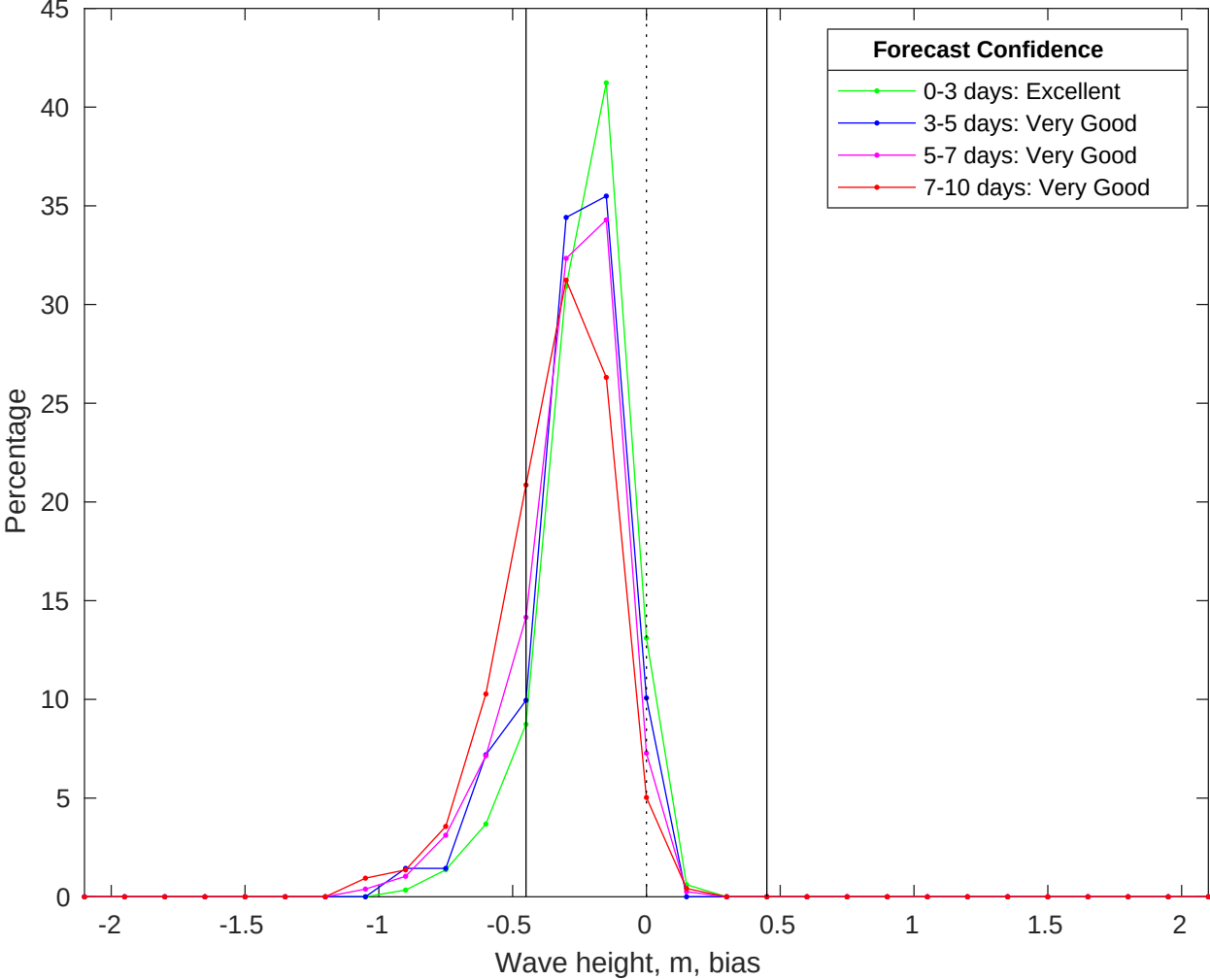
NDBC 52213 vs CMEMS Waves Bias Histogram: 07-Jun-2025
