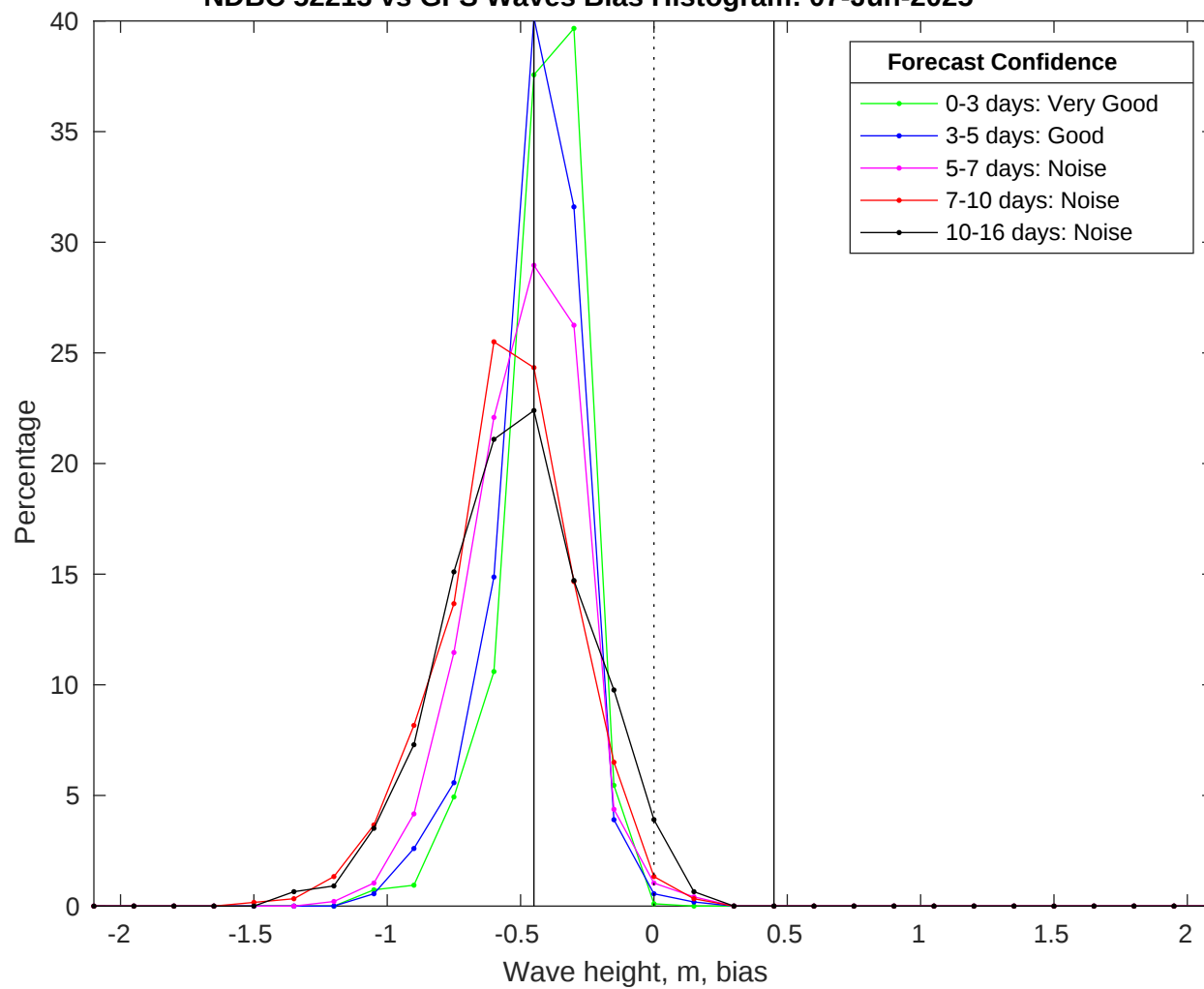
NDBC 52213 vs GFS Waves Bias Histogram: 07-Jun-2025
