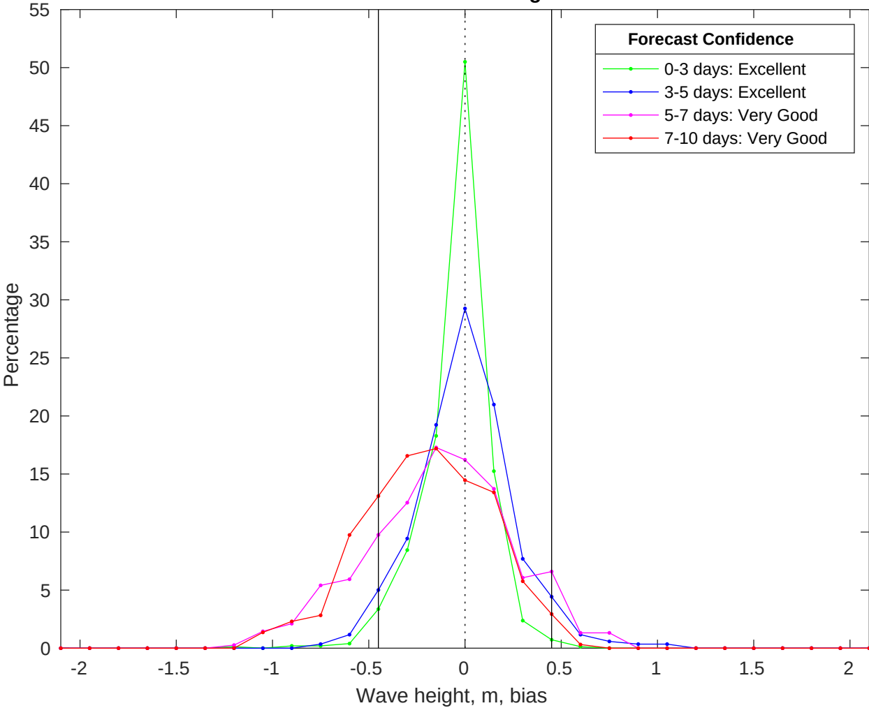
NDBC 41004 vs CMEMS Waves Bias Histogram: 08-Jun-2025
