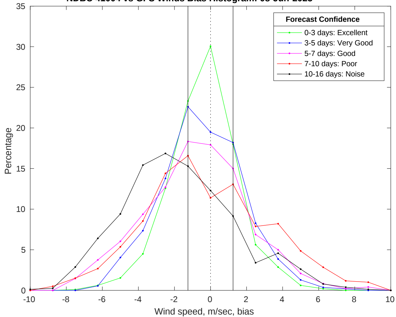
NDBC 41004 vs GFS Winds Bias Histogram: 08-Jun-2025
