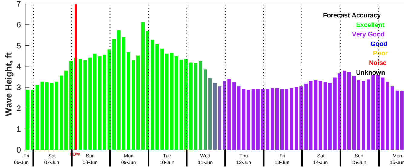
CMEMS Wave Forecast for NDBC 41004 from 06-Jun-2025 19:00:00 to 16-Jun-2025 19:00:00
