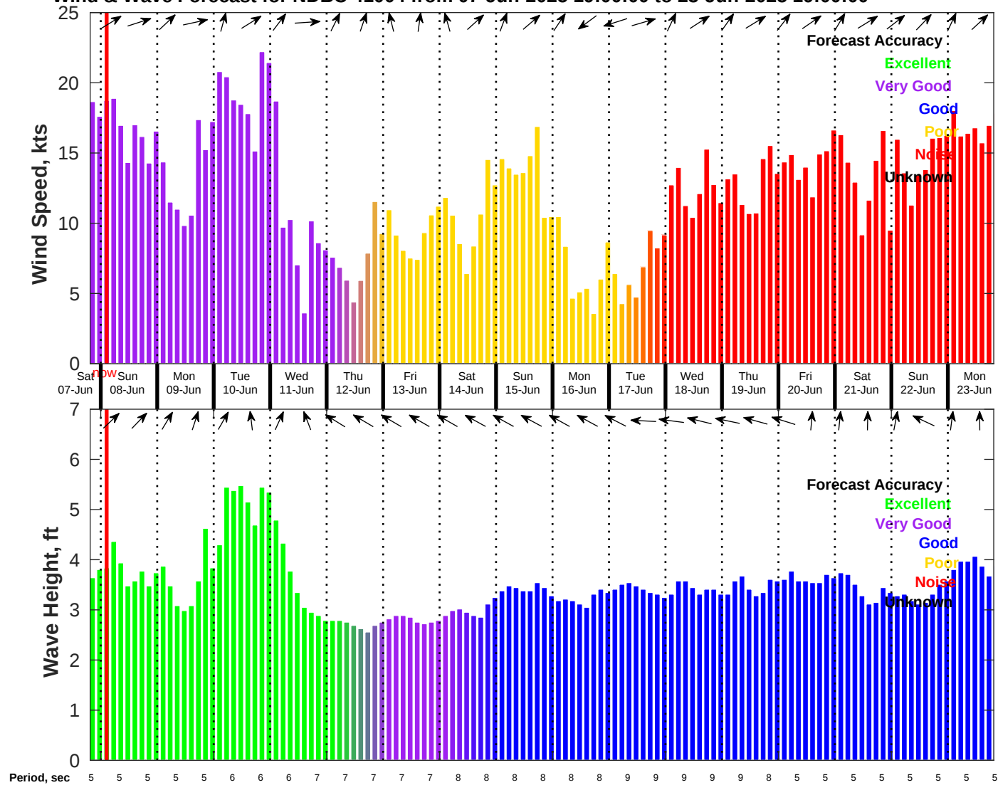
Wind & Wave Forecast for NDBC 41004 from 07-Jun-2025 19:00:00 to 23-Jun-2025 19:00:00
