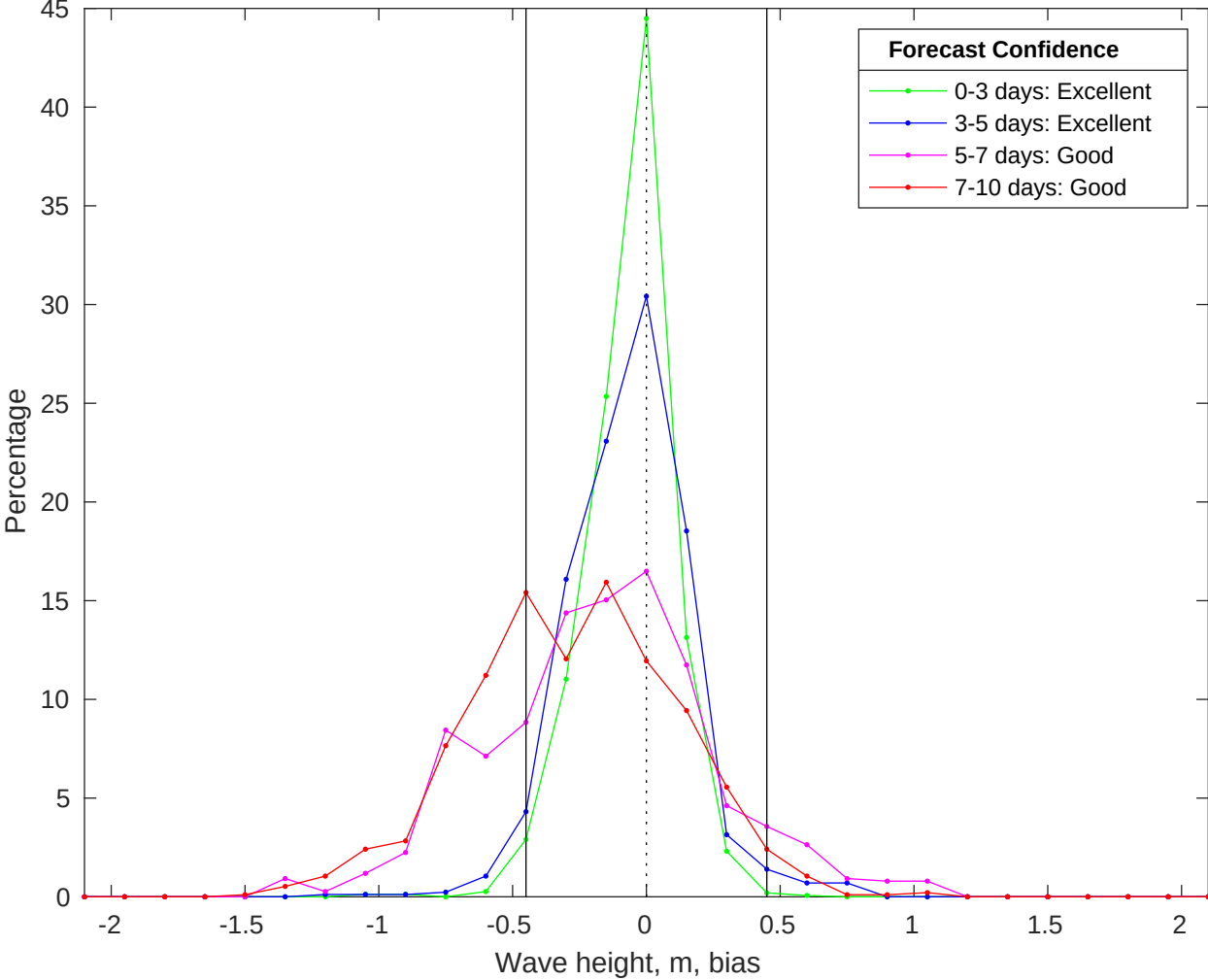
NDBC 41013 vs CMEMS Waves Bias Histogram: 08-Jun-2025
