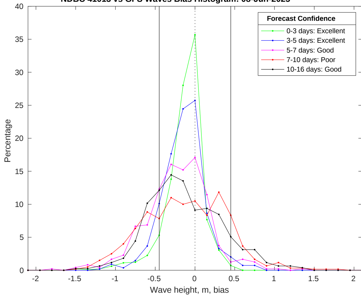
NDBC 41013 vs GFS Waves Bias Histogram: 08-Jun-2025
