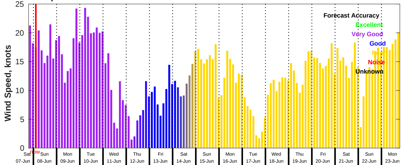
GFS Wind Speed Forecast for NDBC 41013 from 07-Jun-2025 19:00:00 to 23-Jun-2025 19:00:00
