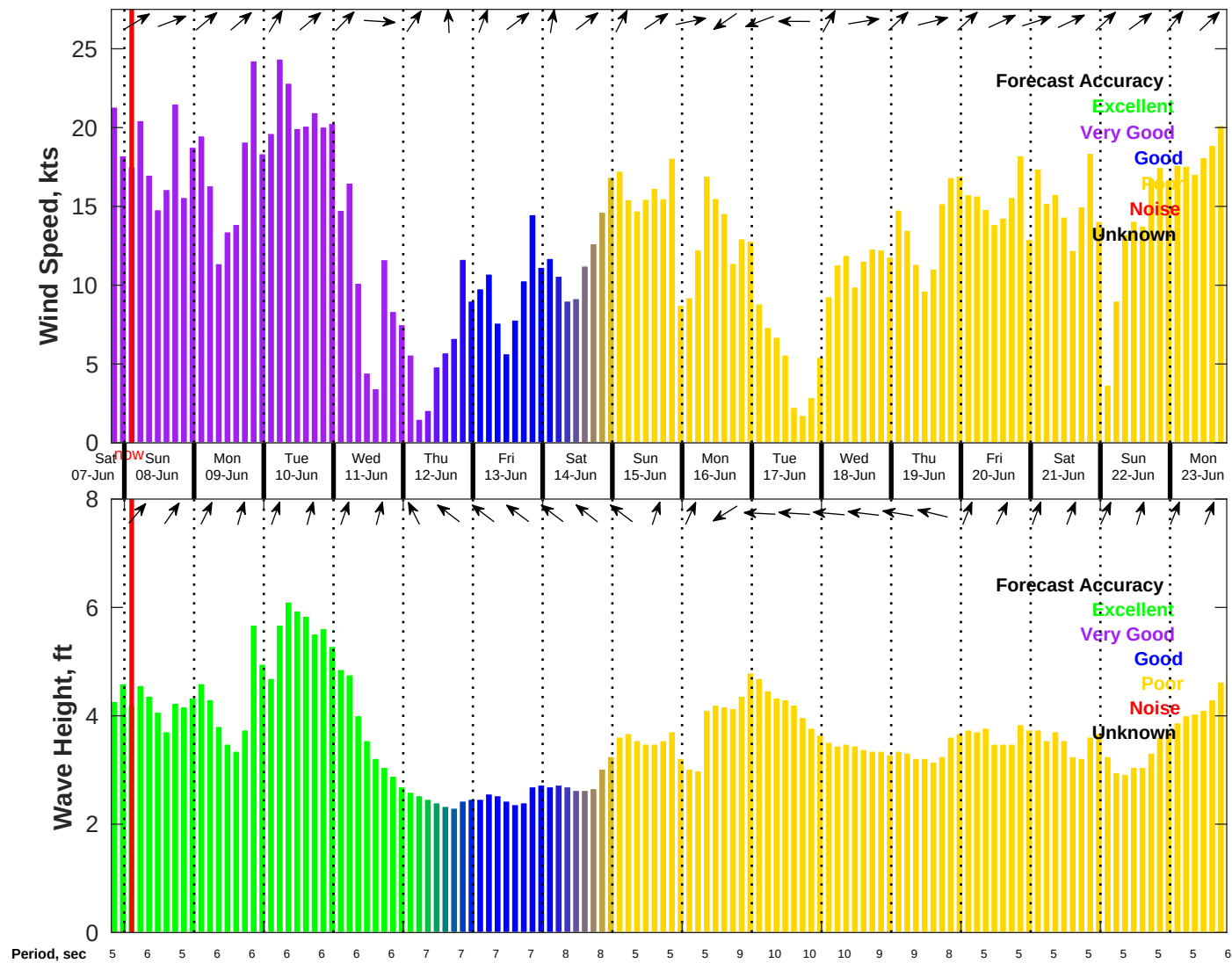
Wind & Wave Forecast for NDBC 41013 from 07-Jun-2025 19:00:00 to 23-Jun-2025 19:00:00
