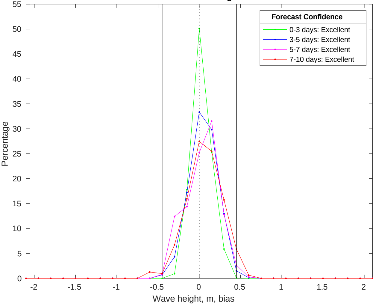
NDBC 41040 vs CMEMS Waves Bias Histogram: 08-Jun-2025
