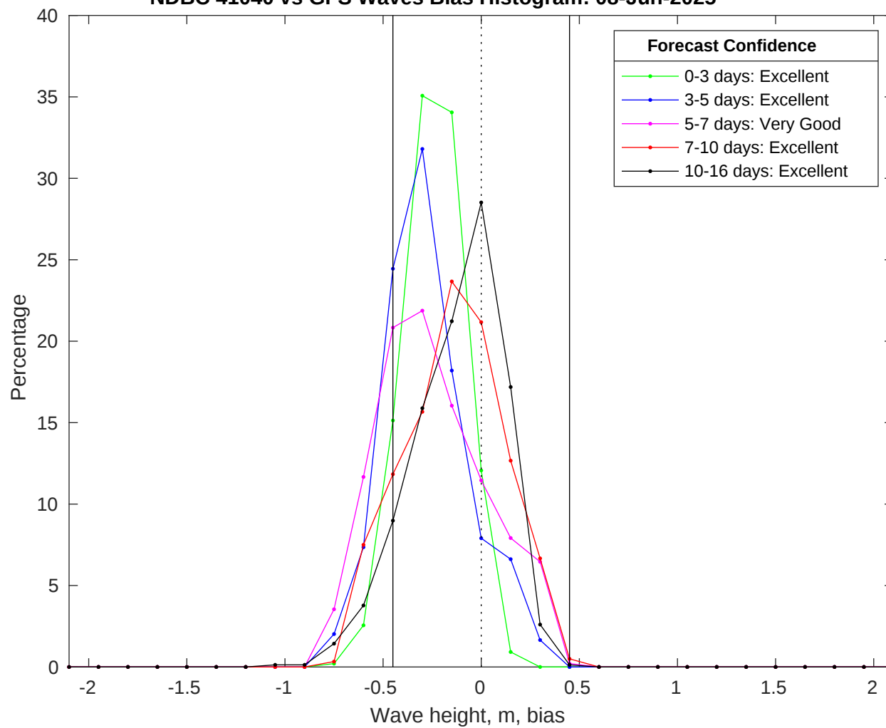
NDBC 41040 vs GFS Waves Bias Histogram: 08-Jun-2025
