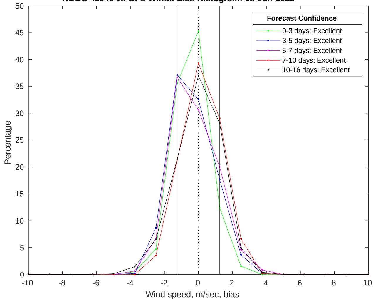
NDBC 41040 vs GFS Winds Bias Histogram: 08-Jun-2025
