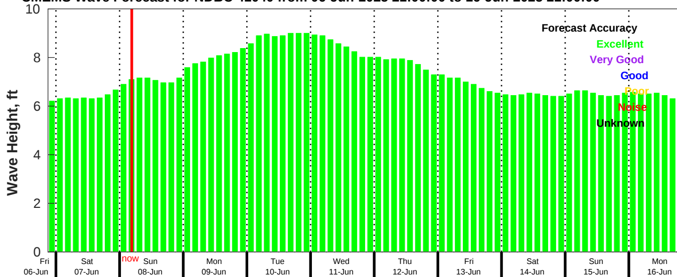
CMEMS Wave Forecast for NDBC 41040 from 06-Jun-2025 21:00:00 to 16-Jun-2025 21:00:00
