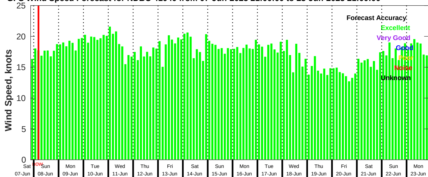
GFS Wind Speed Forecast for NDBC 41040 from 07-Jun-2025 21:00:00 to 23-Jun-2025 21:00:00
