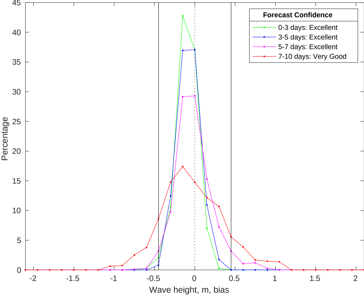
NDBC 42019 vs CMEMS Waves Bias Histogram: 08-Jun-2025
