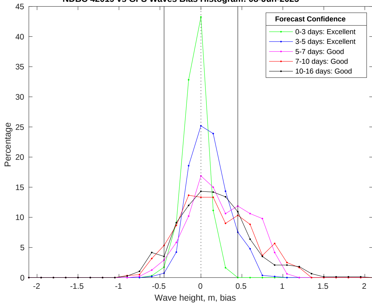
NDBC 42019 vs GFS Waves Bias Histogram: 08-Jun-2025
