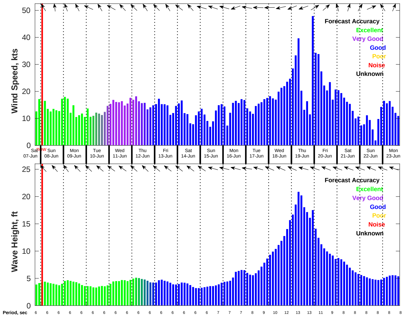
Wind & Wave Forecast for NDBC 42019 from 07-Jun-2025 18:00:00 to 23-Jun-2025 18:00:00
