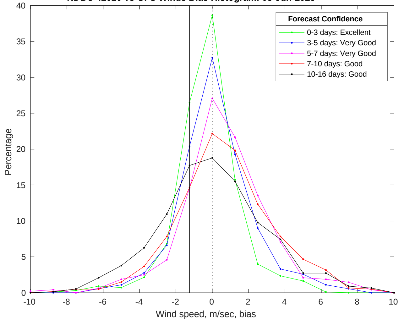
NDBC 42020 vs GFS Winds Bias Histogram: 08-Jun-2025
