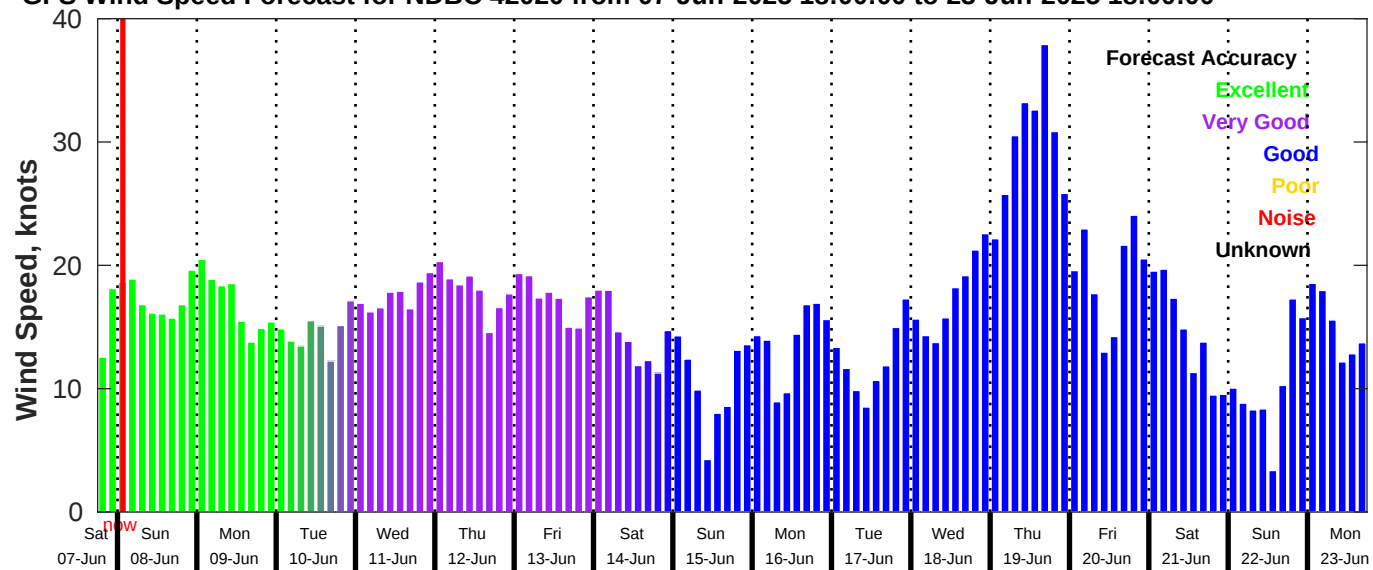
GFS Wind Speed Forecast for NDBC 42020 from 07-Jun-2025 18:00:00 to 23-Jun-2025 18:00:00
