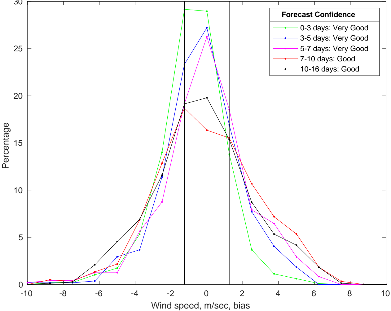
NDBC 42035 vs GFS Winds Bias Histogram: 08-Jun-2025
