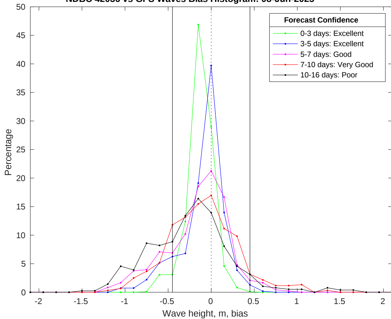
NDBC 42036 vs GFS Waves Bias Histogram: 08-Jun-2025
