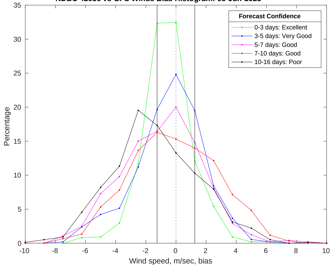
NDBC 42036 vs GFS Winds Bias Histogram: 08-Jun-2025
