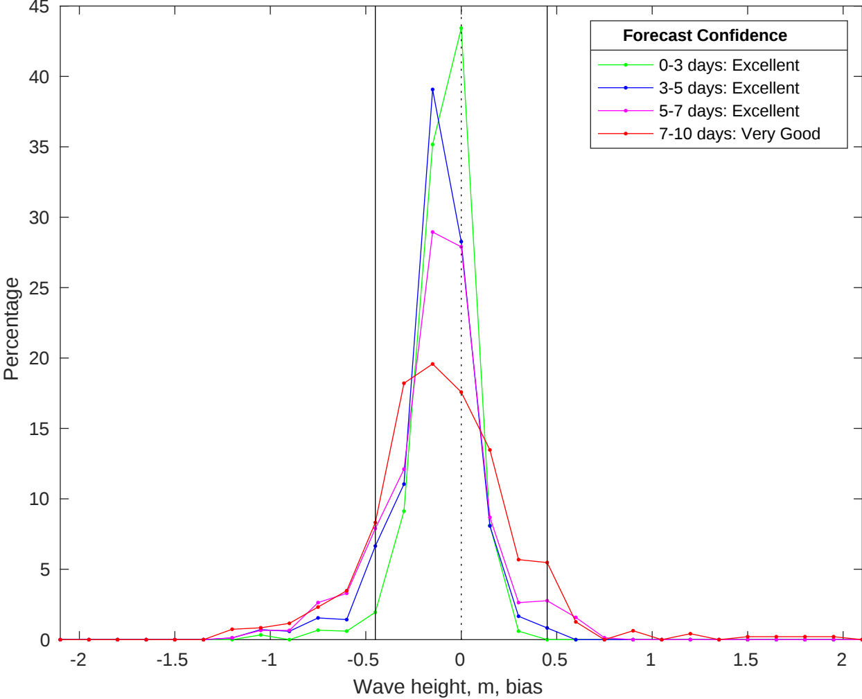
NDBC 42040 vs CMEMS Waves Bias Histogram: 08-Jun-2025
