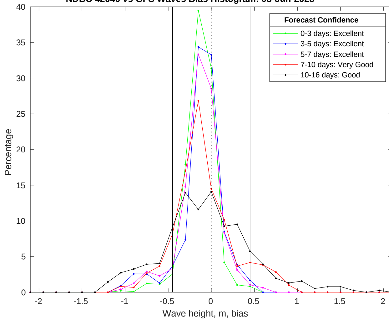
NDBC 42040 vs GFS Waves Bias Histogram: 08-Jun-2025
